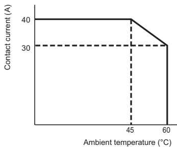
(Fig. 1) Ambient temperature and contact current
